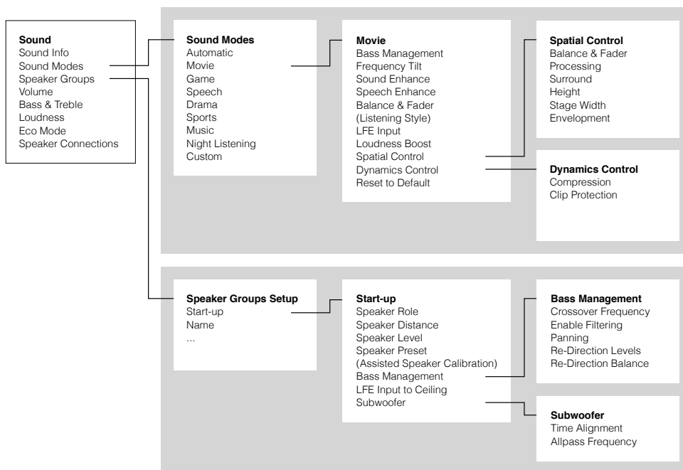
Figure 2.2: Menu map for BeoVision Horizon and BeoVision Avant NG. Note that the list of available features are almost identical to those in Figure 2.3 - only the organisation of items is different. Options marked with parentheses are dependent on the capabilities of the specific system and may not be available on a specific product or software version.
